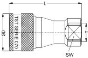
Female Thread Coupler
