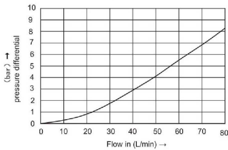
characteristic curves 1=P1-A;B-P2 2=P1-C;D-P2
